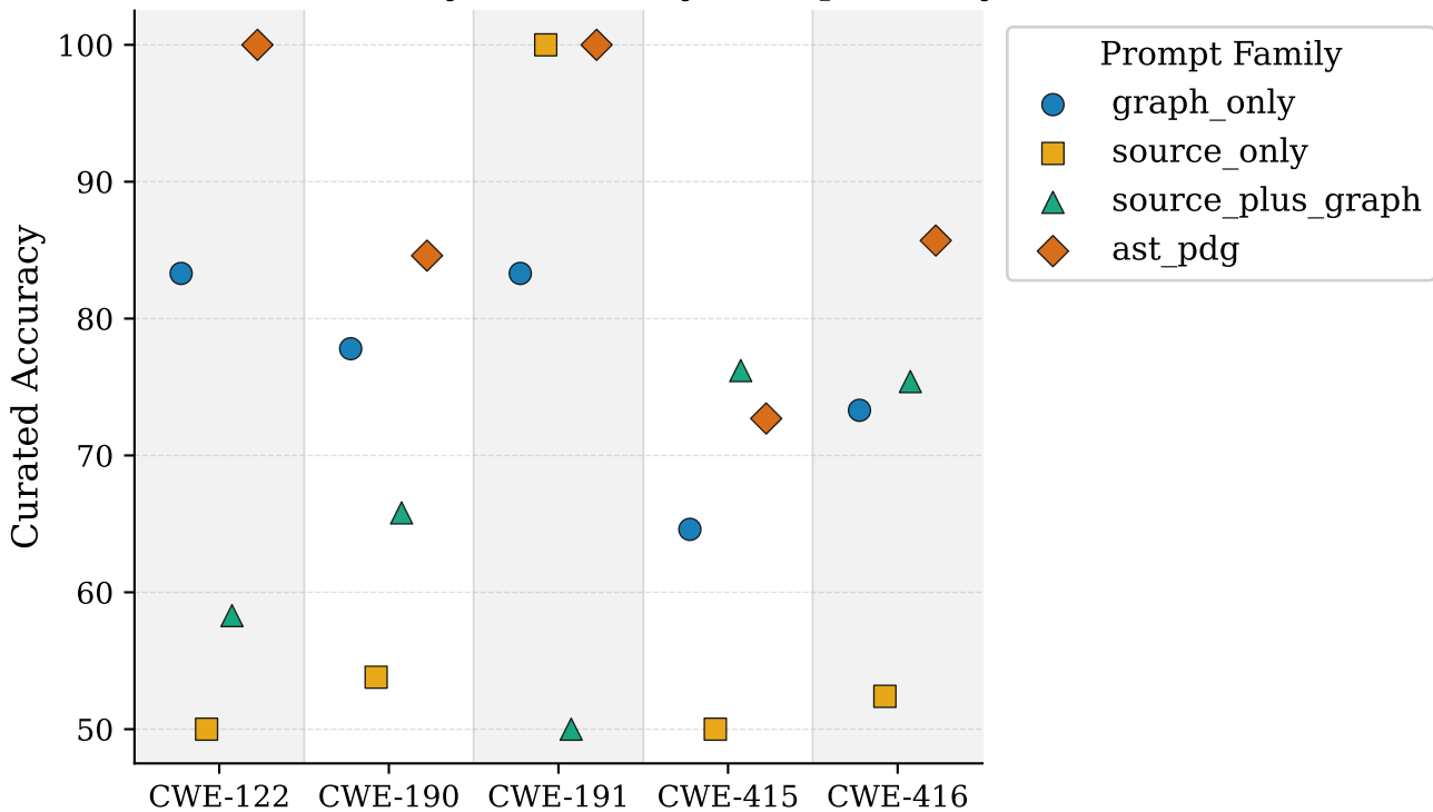
Curated Accuracy vs CWE: by Prompt Family
